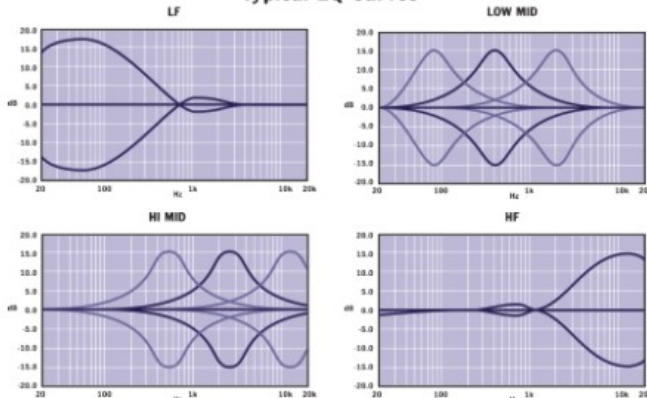
Typical EQ Curves
