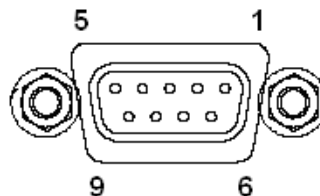
9-pin D-sub Connector Pinout
